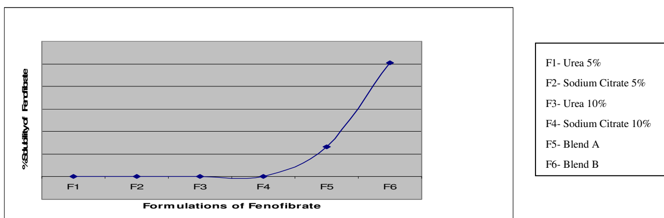
Figure 1. Synergistic effect of hydrotropic reagents on solubility of Fenofibrate
